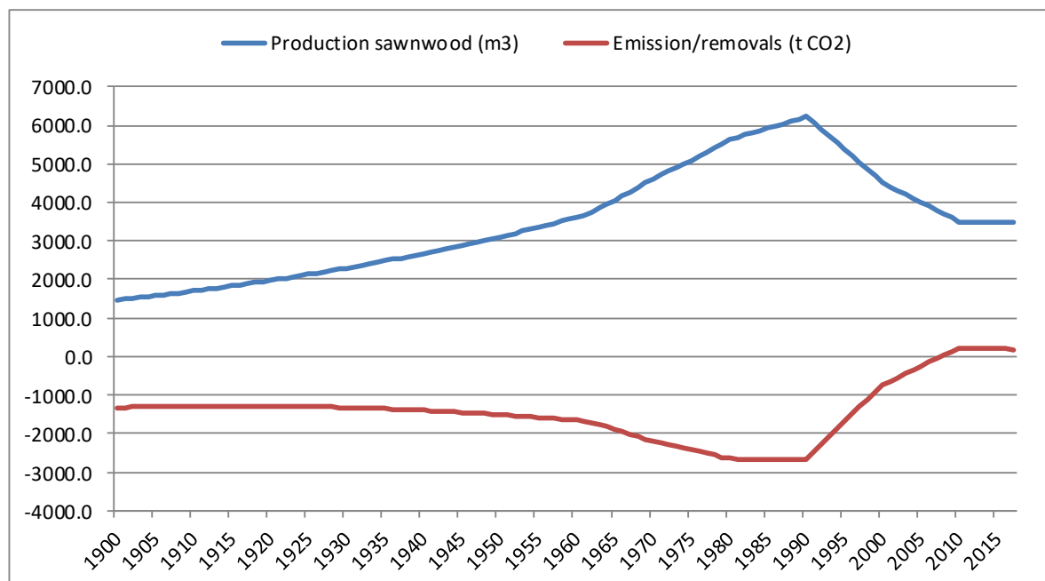
Figure 6-6 Liechtenstein's sawnwood production (m 3 ) and net emissions (positive sign) and removals (negative sign) of CO 2 (tons) from Harvested Wood Products between 1900 and 2017 originating from forest land (UNFCCC) or land under Forest Management (KP).
