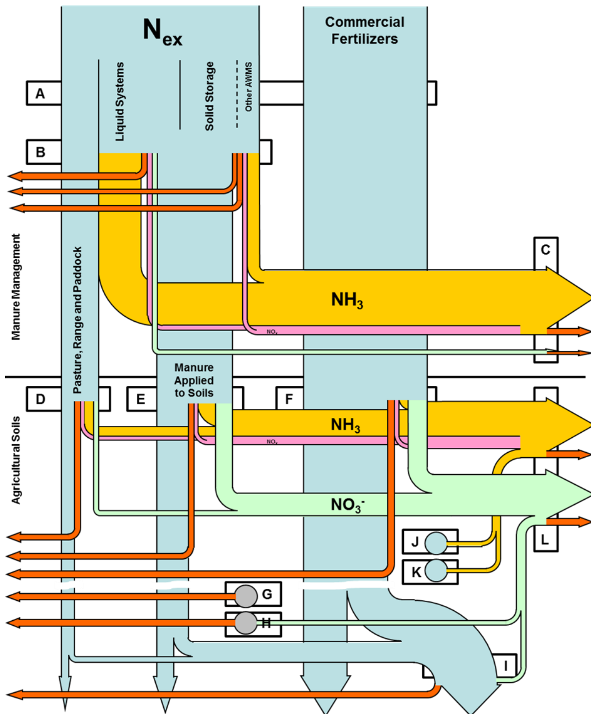
Figure 5-7 Diagram depicting the methodology of the approach to calculate the N 2 O emissions in agriculture (red arrows). Black frames and the respective letters refer to the nitrogen flows in Table 5-18. Note that the figure shows explicitly the methodology of the approach and not necessarily the physical nitrogen flows.
