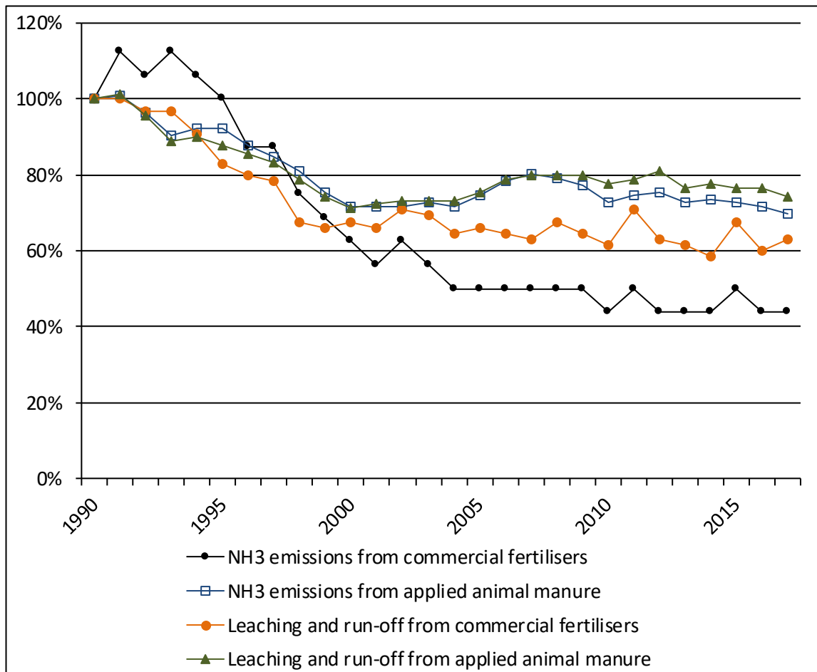
Figure 5-9 Relative development of the most important activity data for source category 3Db indirect N 2 O emissions from managed soils.
