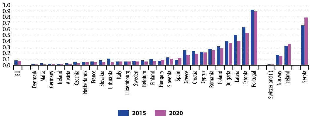
Figure 9.9: Air emissions intensity of industry for particulate matter (PM 2.5 ), by country, 2015 and 2020 (grams per euro, chain-linked volumes, 2010)
