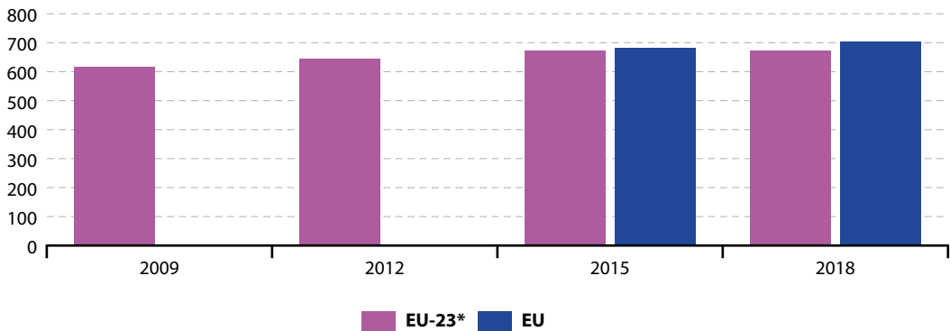
Figure 11.9: Settlement area per capita, EU, 2009–2018 (m 2 )
