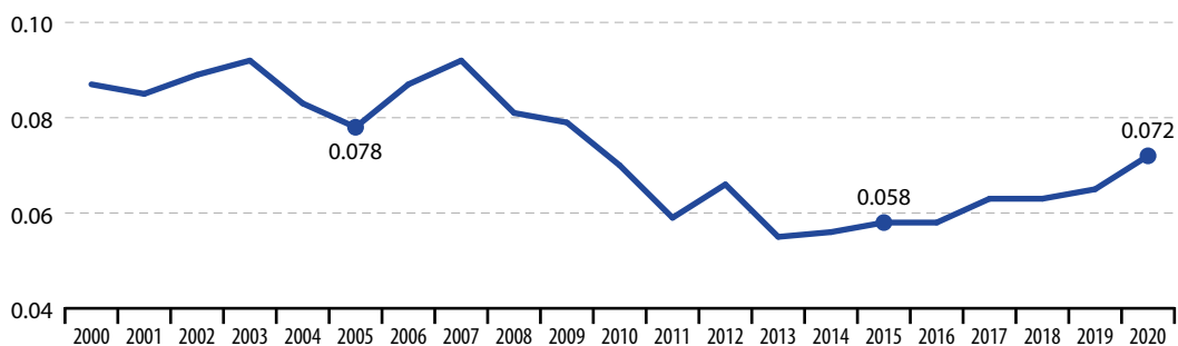
Figure 6.9: Phosphate in rivers, EU, 2000–2020 (mg \text{PO}_4 per litre)
