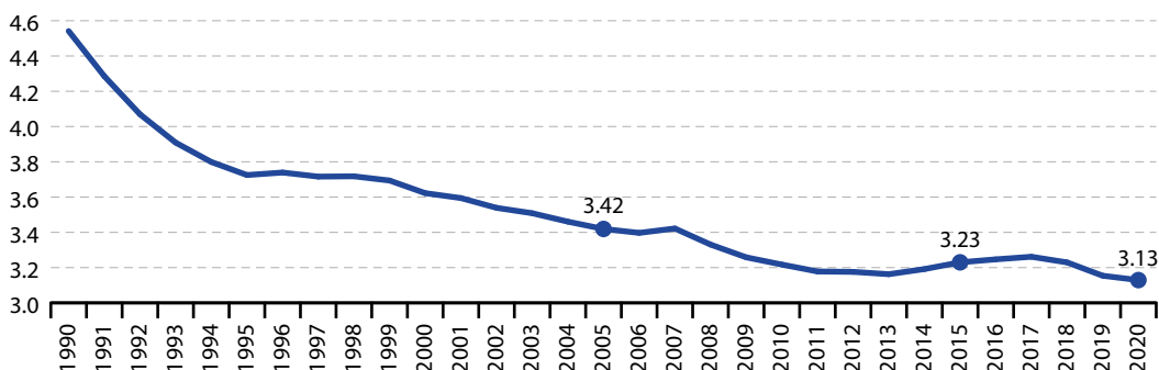
Figure 2.9: Ammonia emissions from agriculture, EU, 1990–2020 (million tonnes)
