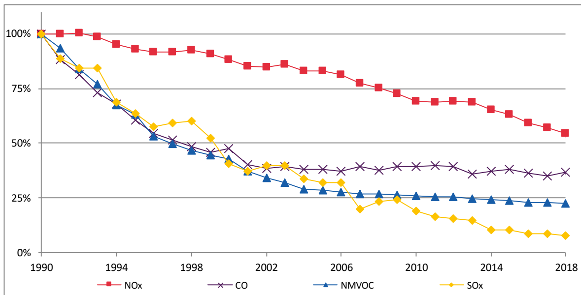
ES Figure 3 Trend of NO x , CO, NMVOC and SO x emissions as of CLRTAP submission 2020 (OE 2020f).
