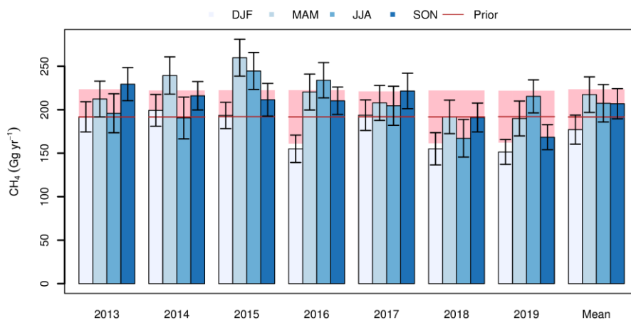
Figure A – 14: Seasonality of Swiss CH 4 emissions. A priori values and their uncertainties are given as red lines and red shaded areas. A posteriori emissions are given as blue bars and uncertainty bars for different seasons (DJF: December, January, February; MAM: March, April, May; JJA: June, July, August; SON: September, October, November). All uncertainties refer to 1- \sigma confidence intervals.
