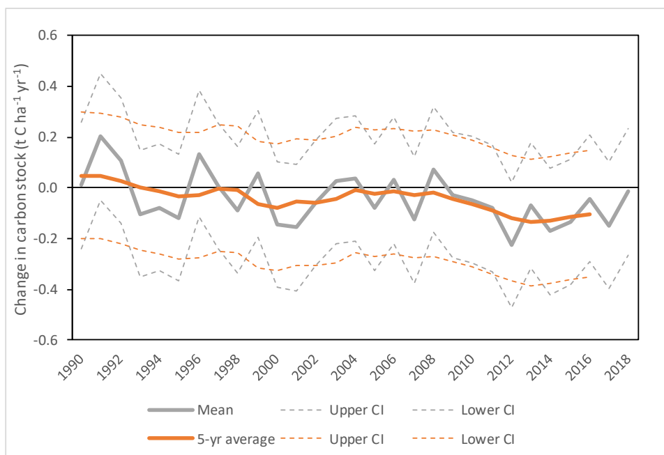
Figure 6-12 Annual carbon stock changes ( \text{t C ha}^{-1} \text{ yr}^{-1} ) and corresponding 5-year moving averages in mineral soil (0-30 cm) for permanent grassland (CC31), area-weighted across three elevation zones, plus upper and lower confidence intervals (see chp. 6.6.3). The 5-year averages are displayed to highlight the trends; they are not used for the reporting.
