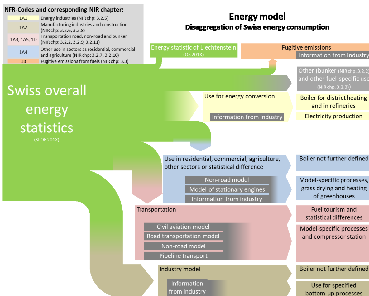
Figure 3-9 Overview of Switzerland's energy model. In the abbreviations SFOE 201X and OS 201X the "X" refers to the latest edition of the respective statistics.
