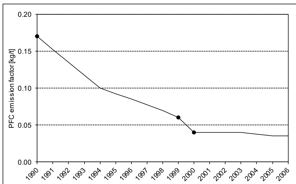
Figure 4-6 Extrapolation of PFC emission factor based on measurements in 1990, 1999 and 2000. The path for the reduction between measurements and the stagnation after the last measurements reflects the observed development of average EFs in the European Union.
