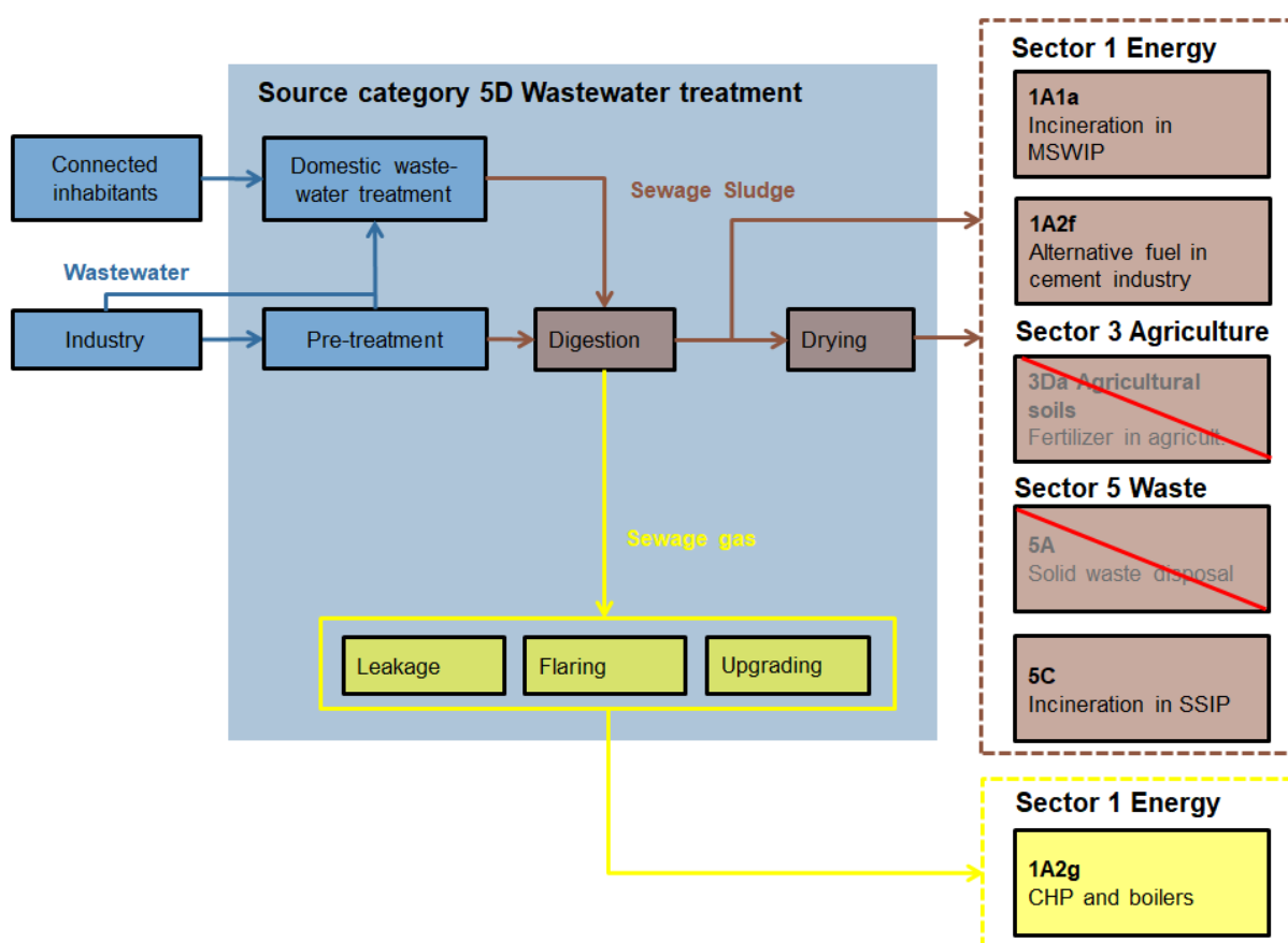
Figure 7-6 System boundaries of processes related to wastewater treatment. CHP = Combined heat and power generation. MSWIP = Municipal solid waste incineration plant. SSIP = Sewage sludge incineration plant.
