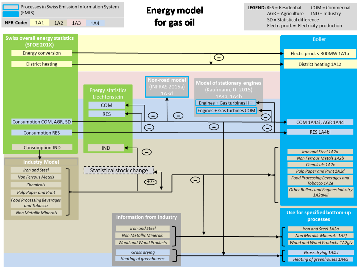
Figure 3-13 Schematic disaggregation of fuel consumption for gas oil. The Swiss overall energy statistics provides gas oil use for energy conversion and the amount thereof being used for district heating. Based on this information, gas oil use is split into 1A1ai Electricity generation and 1A1aiii Heat plants. According to the non-road model, a small amount of gas oil is consumed in source category 1A3d navigation (steam-powered vessels).
