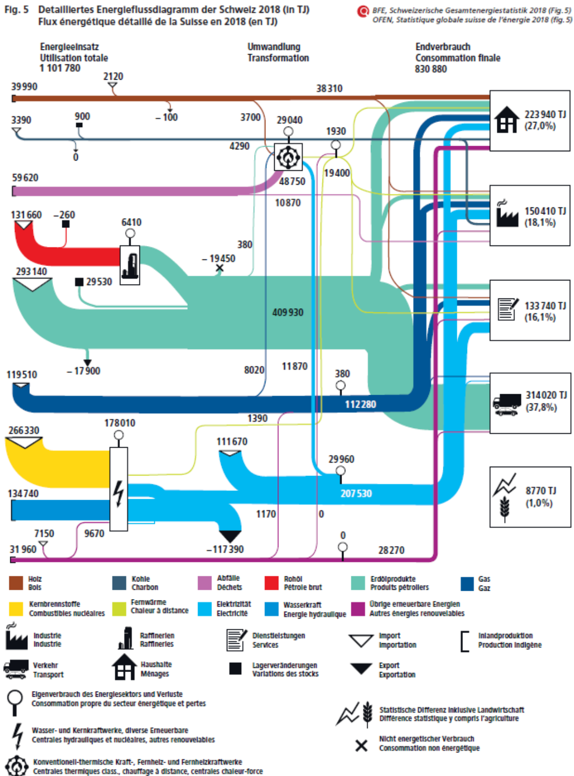
Figure A – 2 Energy flow in Switzerland 2018 in TJ (SFOE 2019)
