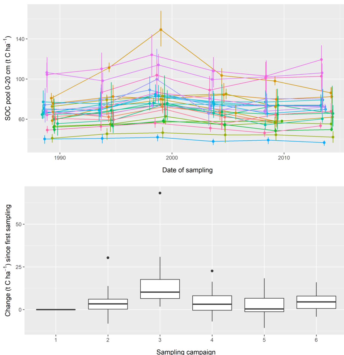
Figure 6-7 Measured SOC pools for topsoils (0–20 cm) and their changes for 27 NABO long-term monitoring sites in forest during the time period 1985–2014. The elevation of the sites ranges from 383 to 1690 m a.s.l. Top panel: SOC pools 0–20 cm per site and sampling; the dots indicate the mean and the bars the range of 5% and 95% percentiles of bootstrap samples taking into account the variability in SOC contents of the individual replicates per site and sampling as well as the variations of the bulk density. Bottom panel: boxplot of changes in SOC pools since first sampling (boxes indicate the lower and the upper quartiles with the median indicated; lines include all observations inside the range of 1.5 times the interquartile distance, observations beyond that range are indicated as dots).
