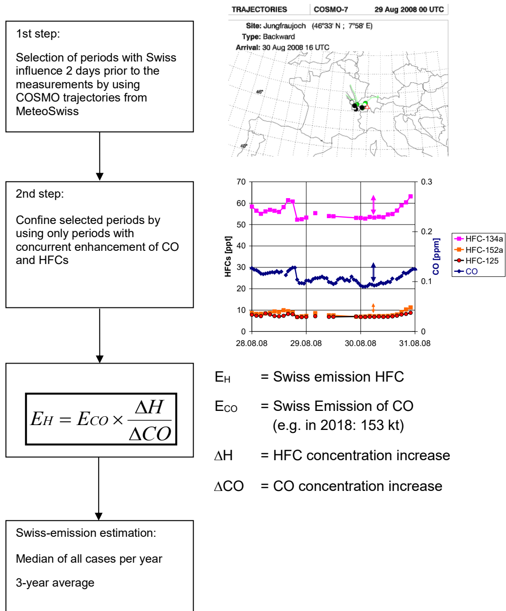
Figure A – 3 Description of the procedure to estimate annual emissions of HFCs from Switzerland by using continuous measurements of HFCs at Jungfrauoch (Switzerland).
