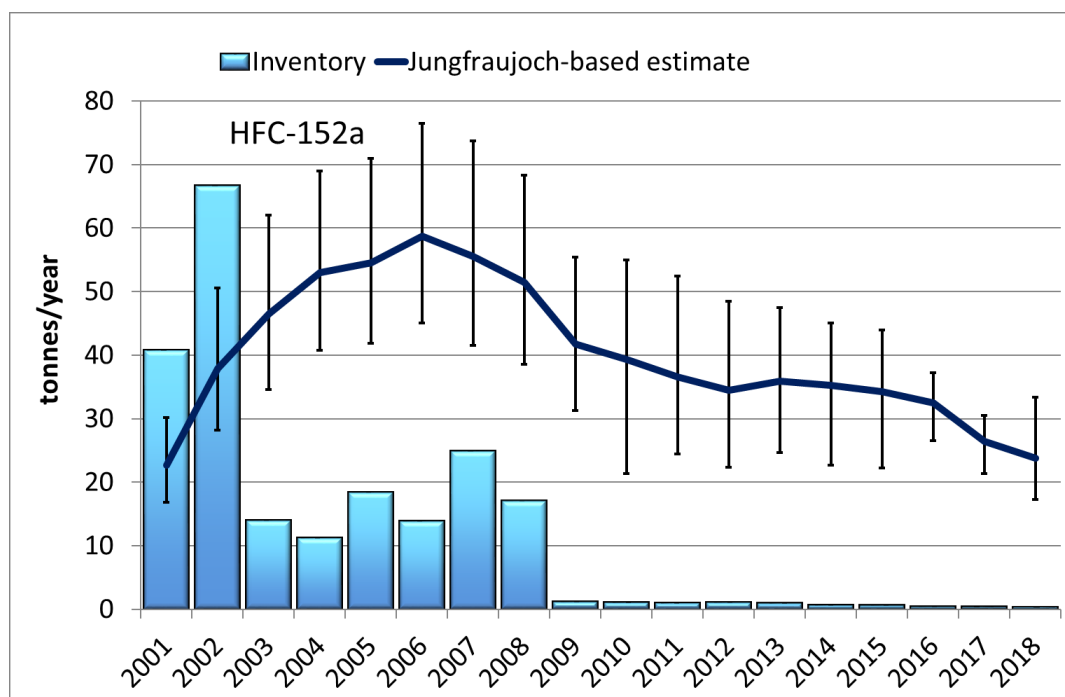
Figure A – 6 Comparison of HFC-152a emissions from Switzerland: Inventory and estimates from measurements at Jungfrauoch.
