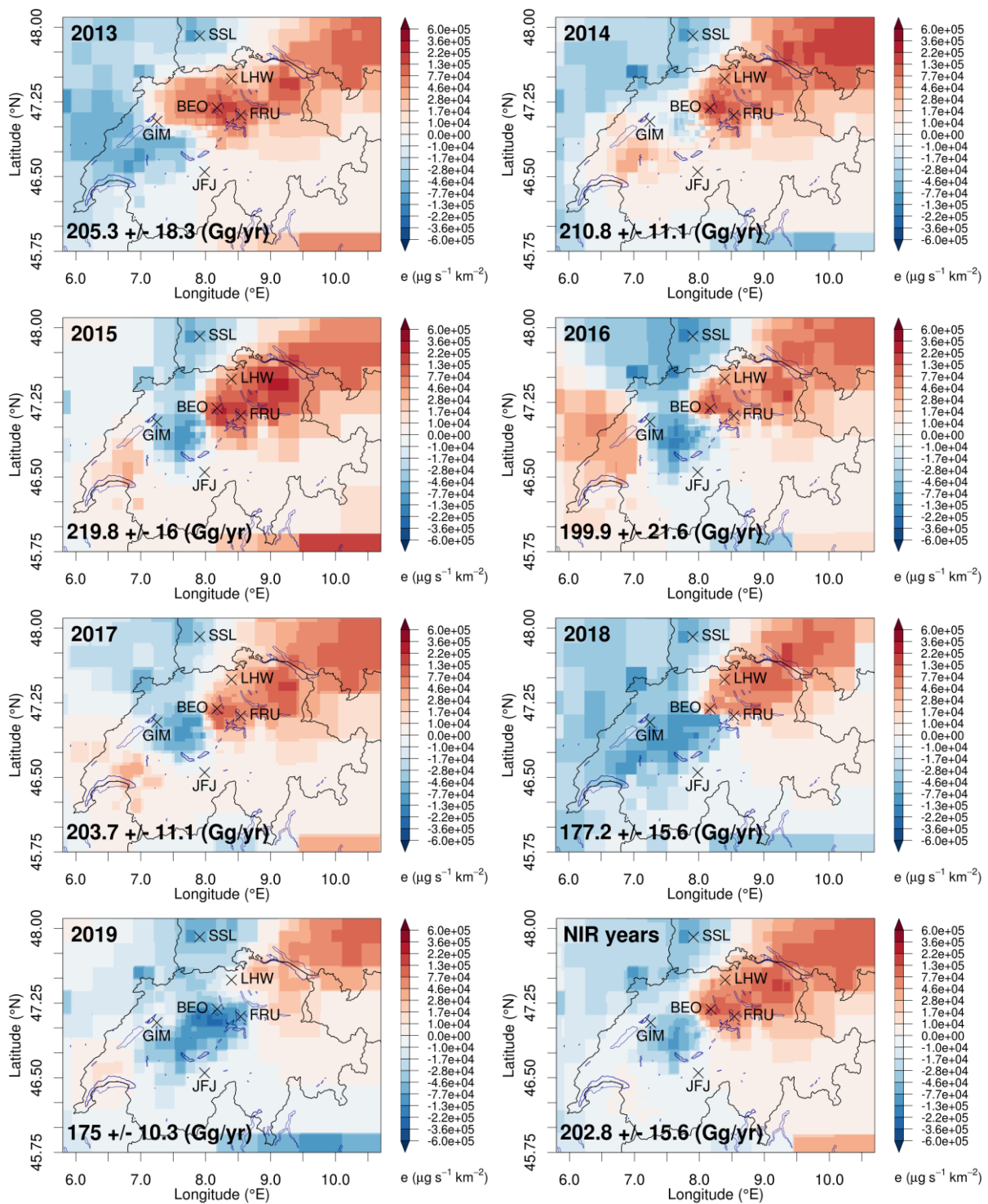
Figure A – 13: Absolute difference between a posteriori and a priori mean annual emissions (each being the mean over 8 sensitivity runs). The numbers given in the plots refer to the total a posteriori Swiss emissions and their uncertainty ( 1\sigma level) for the given year. NIR years refers to the years covered by the latest NIR (2013 to 2018) and gives the according mean estimates and uncertainties.
