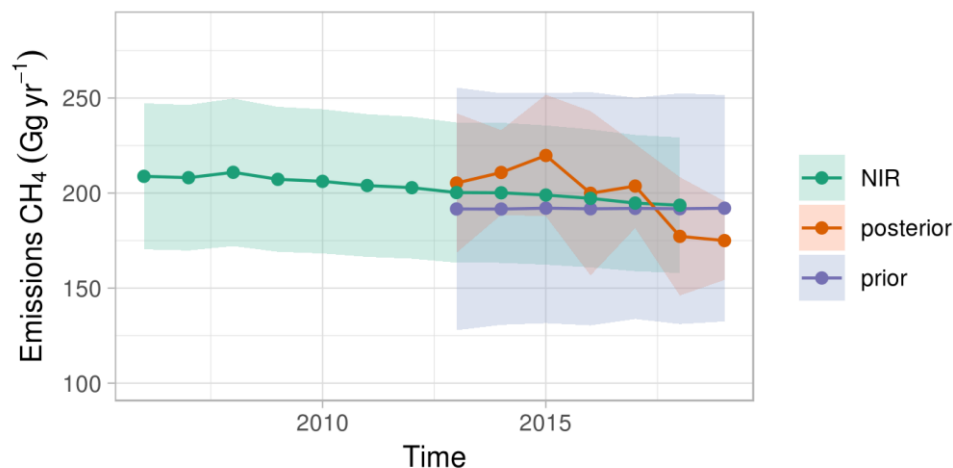
Figure A – 11: Time series of total Swiss CH 4 emissions as reported in the latest NIR (green), used as a priori information in the inverse modelling (purple), and as estimated by the inverse modelling ( a posteriori , orange). The uncertainty ribbons give the 95% confidence (2σ) level of each estimate.
