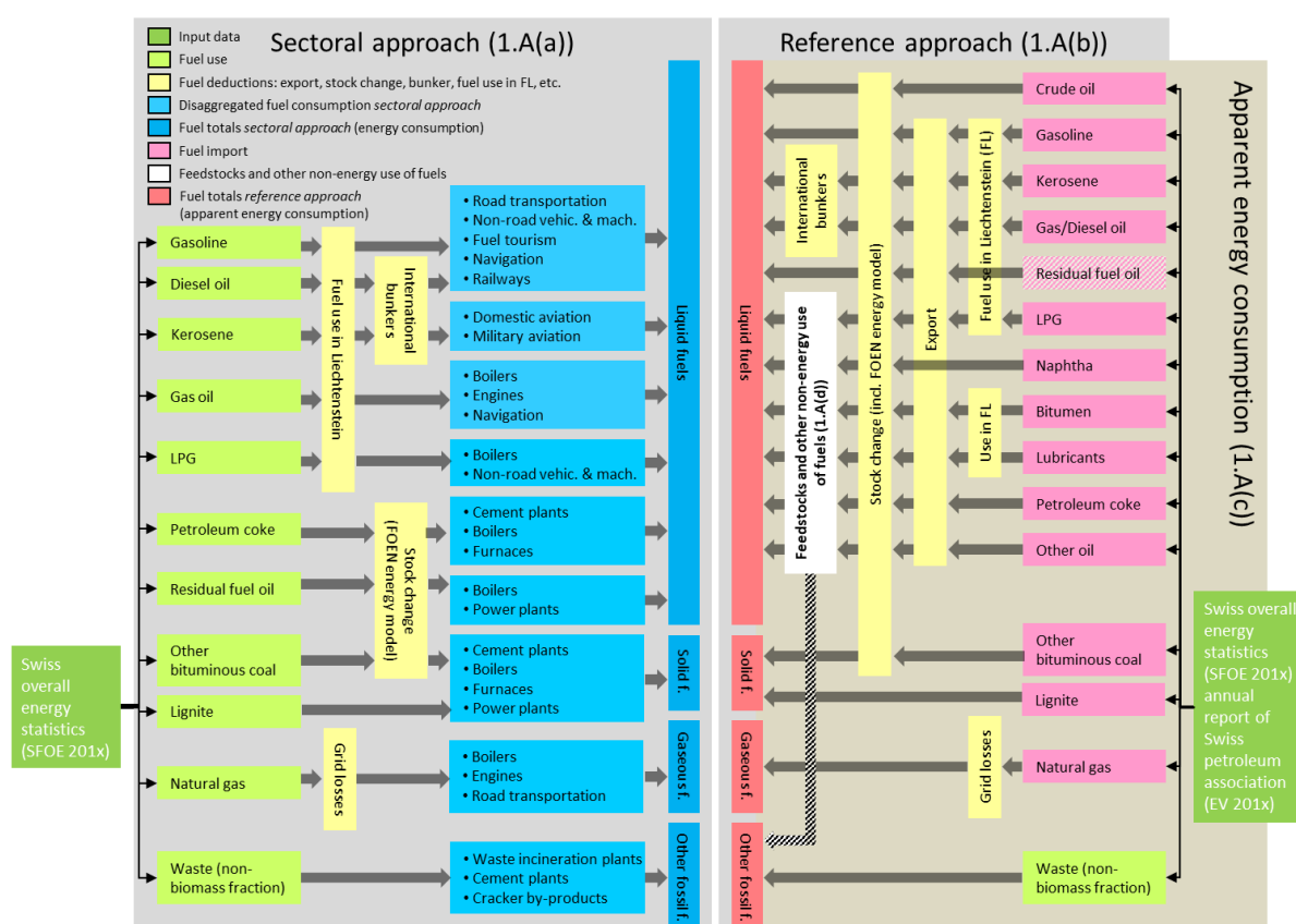
Figure 3-5 Calculation of Reference and Sectoral Approach. The input data for both approaches stem from the Swiss overall energy statistics (SFOE 2019). For the Reference Approach, additional information from Avenergy Suisse (formerly Swiss Petroleum Association) (EV 2019) is used. While the Reference Approach considers the net import/export balance, the Sectoral Approach considers the fuel consumption. The dark grey arrows represent fuel deductions where occurring. The dashed arrow from the Feedstock use to Other fossil fuels stands for the CO 2 emissions from cracker by-products (originating from feedstock use of LPG and naphtha) which are accounted for under Other fossil fuels. The graphic box of the import of Residual fuel oil is dashed since there is no more import of residual fuel oil.
